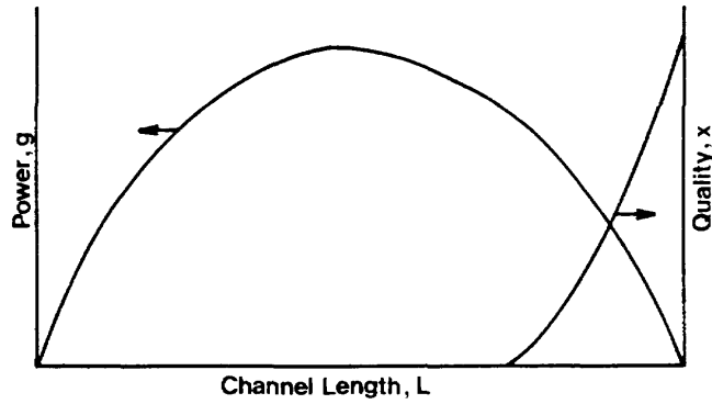
Figure 7.12 Power and quality versus length along a fuel channel.
