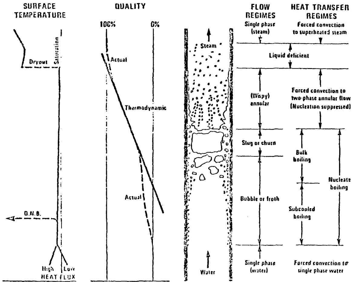
Figure 7.11 Possible thermohydraulic regimes in a coolant channel.
