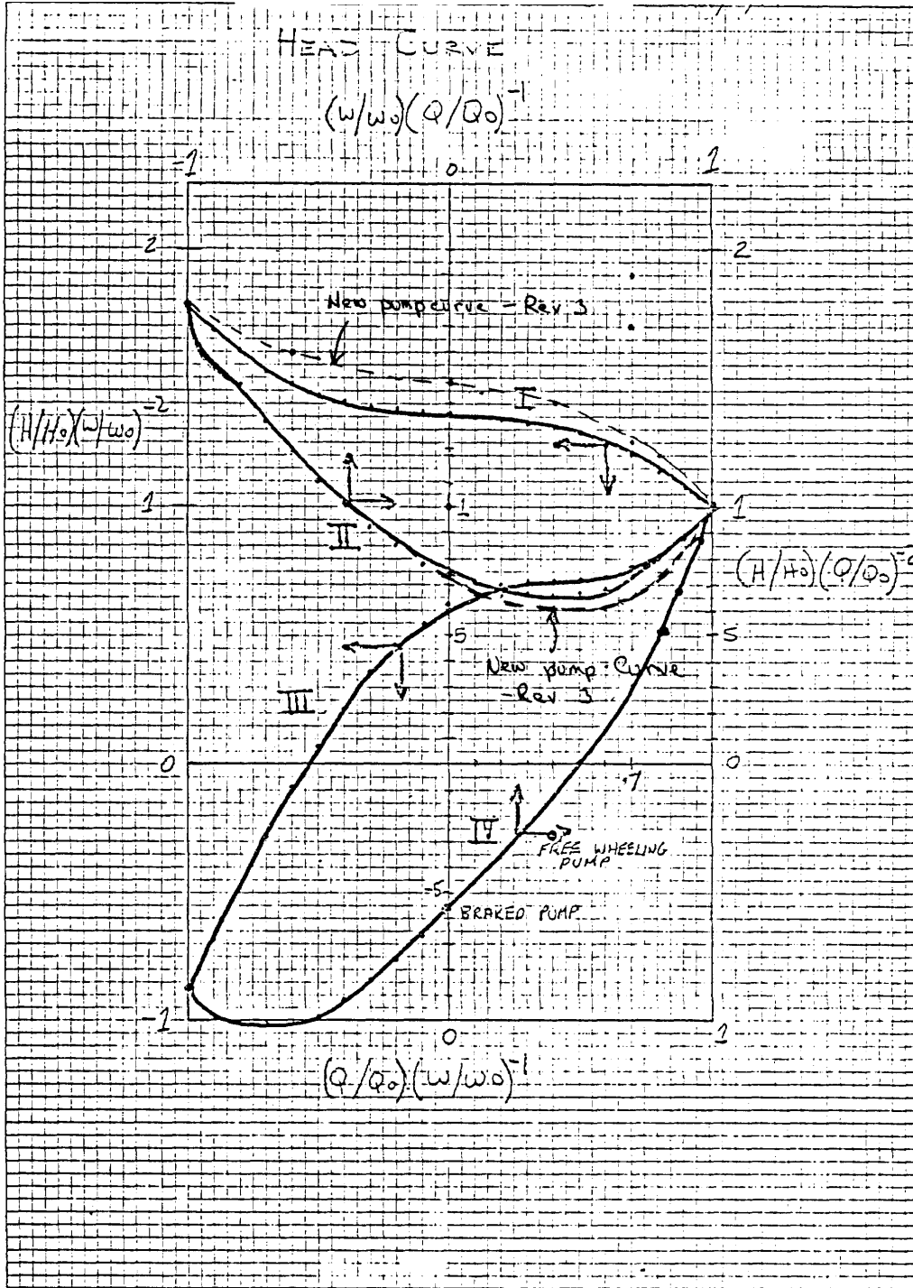
Figure 7.6 Head characteristics for a typical CANDU pump.
