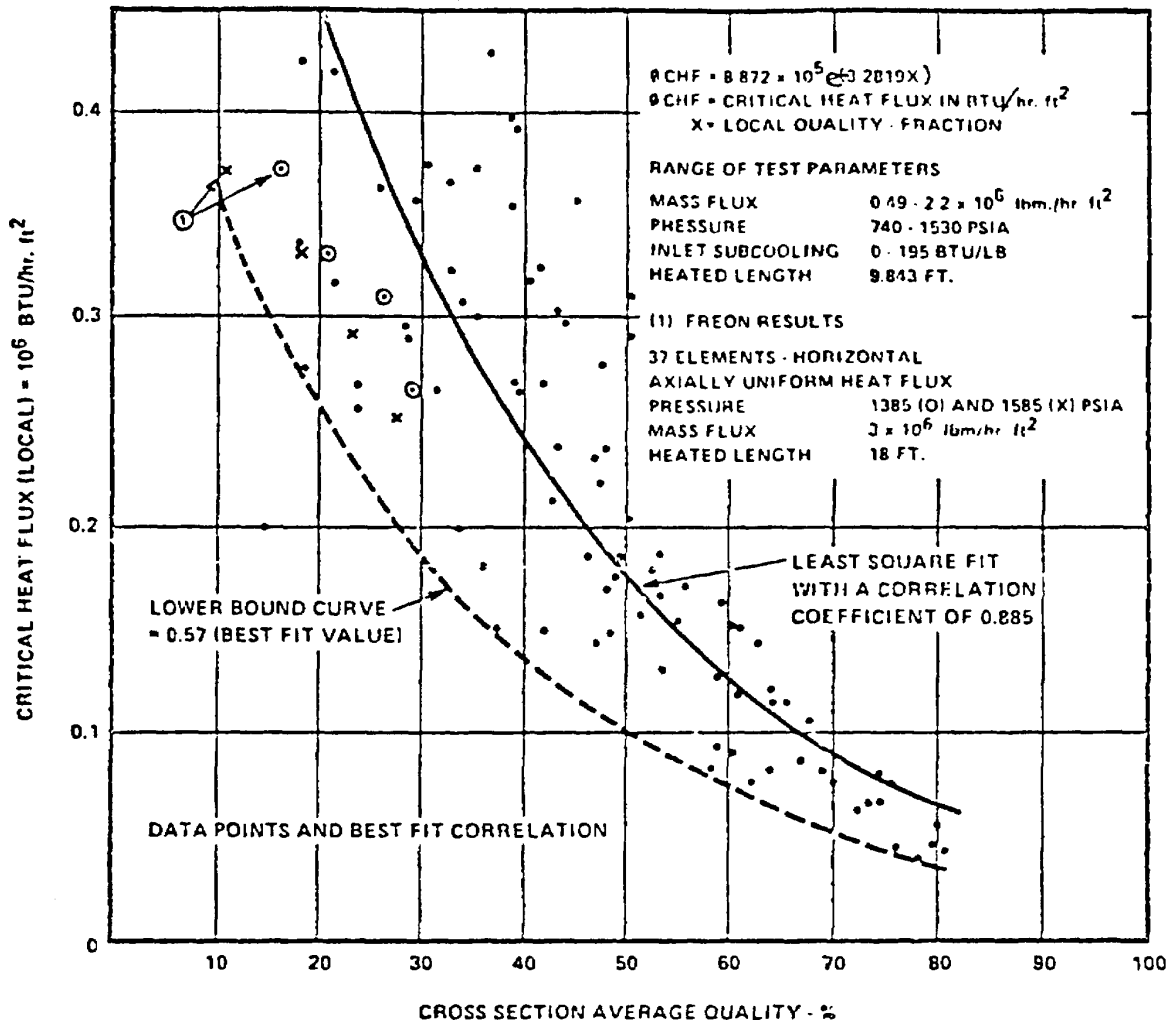
Figure 7.10 Critical heat flux.
