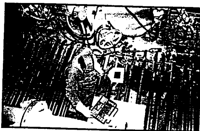
Fig. 3 — The welding operator controls the welding operation from the pendant while the weld head, which is positioned on the bottom row of the superheater header tubing, executes the weld.
