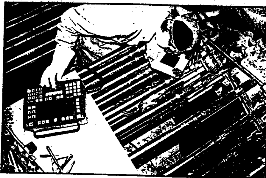
Fig. 2 — An orbital welding machine operator uses a program operator pendant to adjust the position of the weld head in preparation for welding the superheater header tube. Note the finished chromium-molybdenum-to-chromium-molybdenum welds and the layered arrangement of the tubing entering the superheater header.
