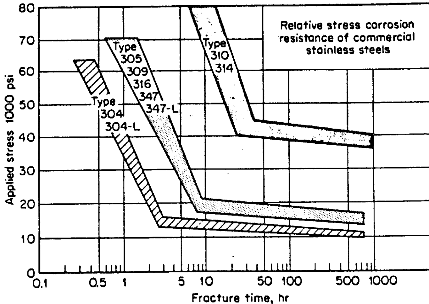
Composite curves illustrating the relative stress corrosion-cracking resistance for commercial stainless steels in boiling 42% magnesium chloride .
