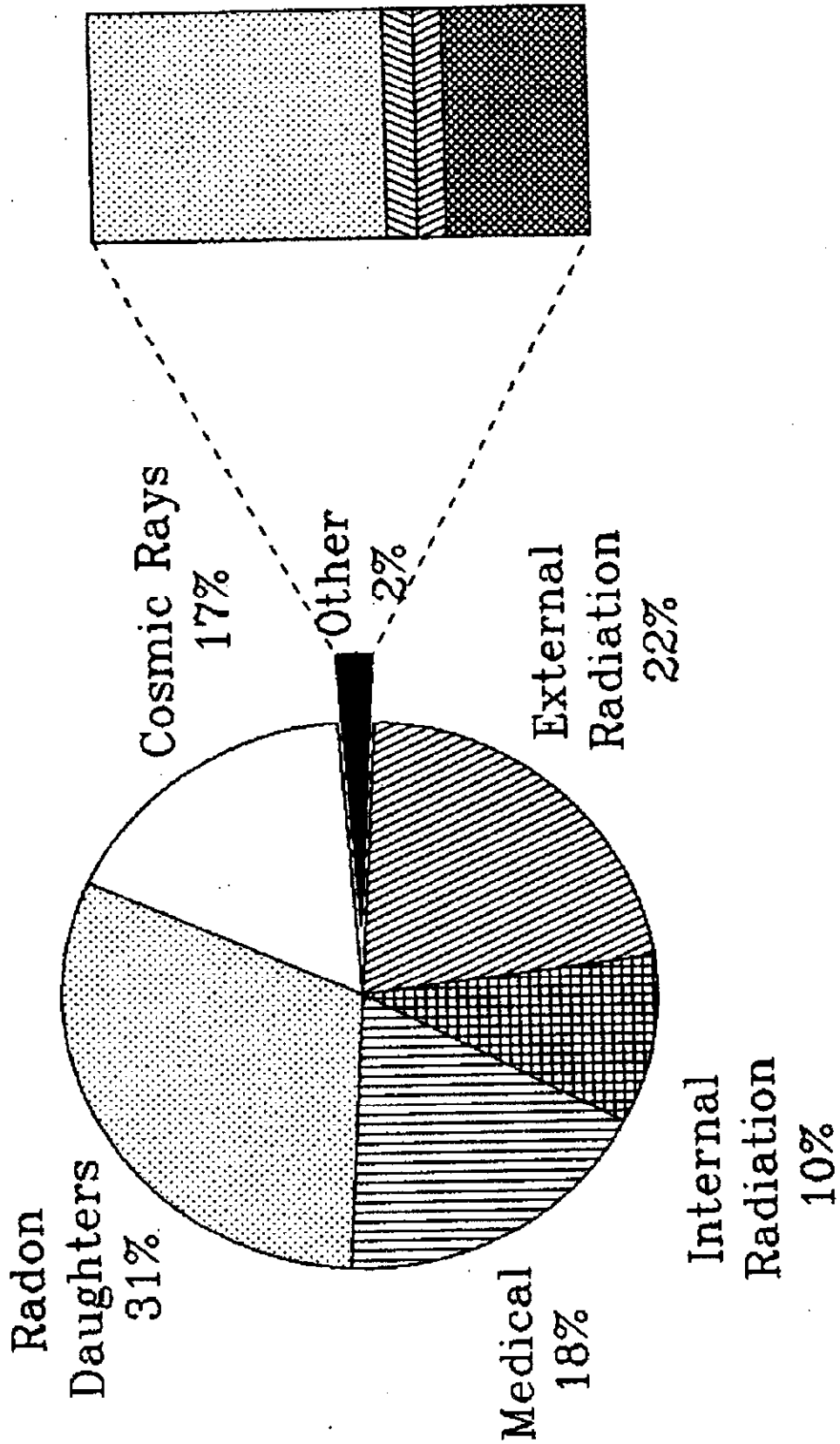
Fig. 3.4. Background Radiation in Canada
