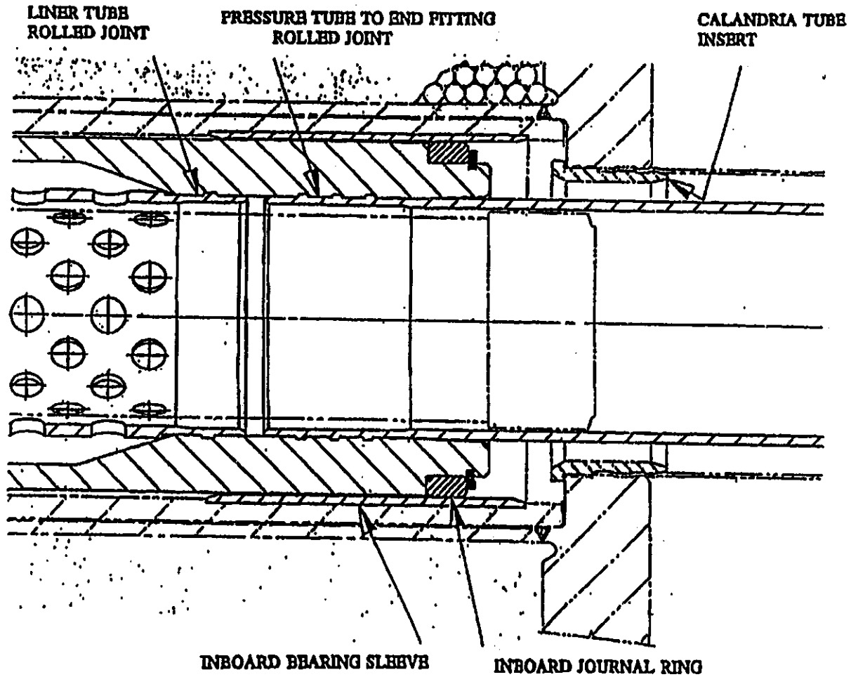
Figure 5-2 Pressure Tube-to-End Fitting Rolled Joint and Inboard Bearing
