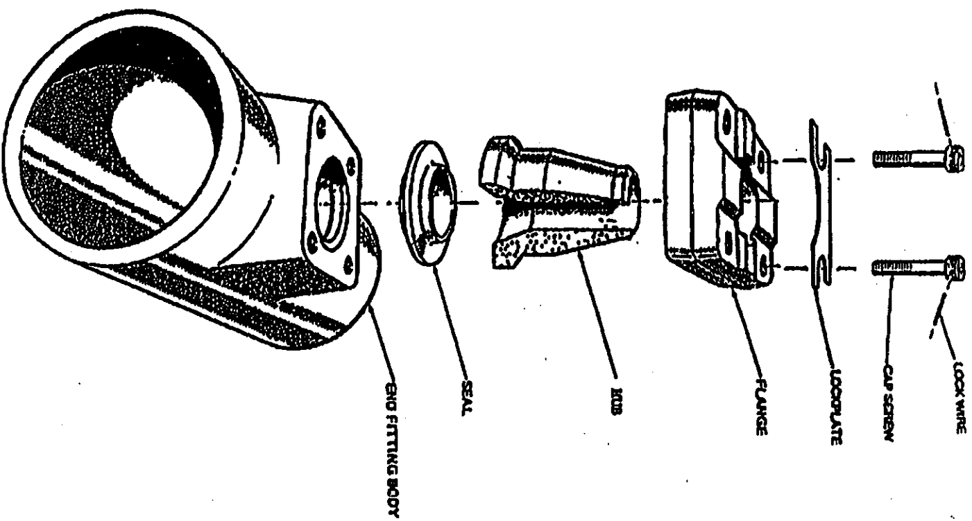
Figure 5-4 Feeder Connection
