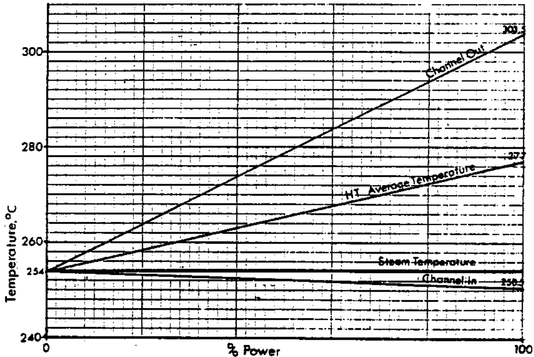
Figure 7 Temperature vs % Full Power
