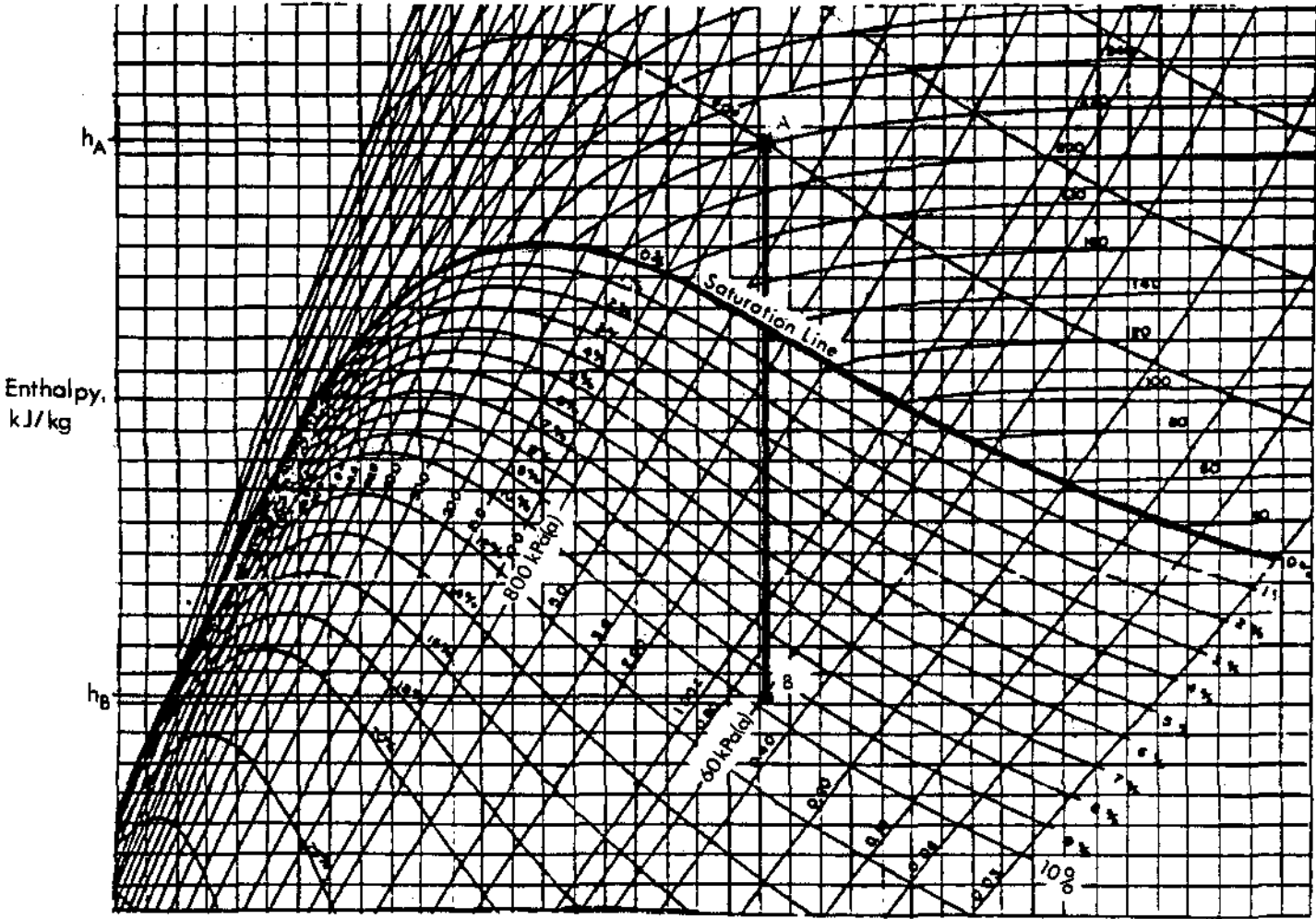
Entropy, kJ/kg°C Fig. 6.3
