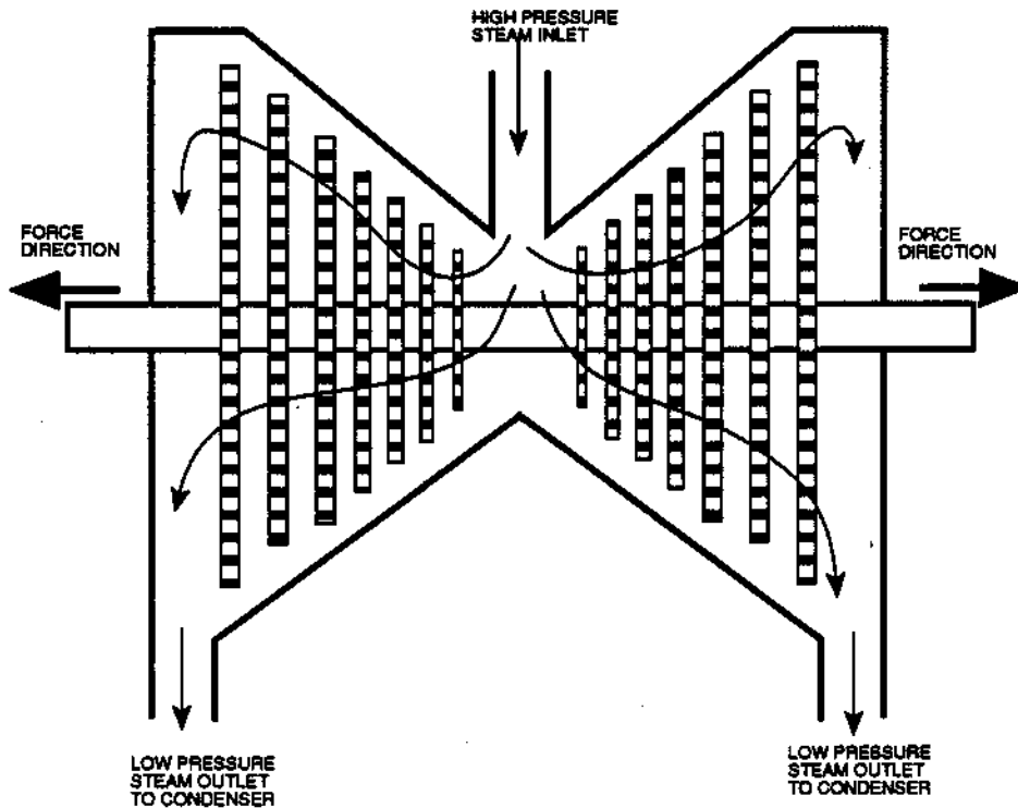
Figure 3.10 Double Flow Turbine
