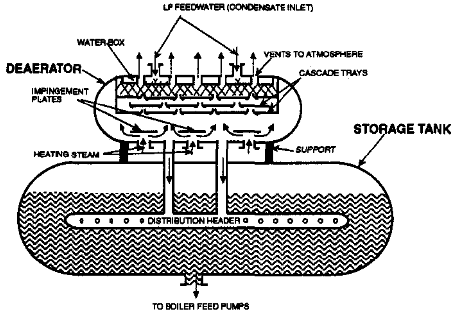
Figure 3.13 Simplified Deaerator and Storage Tank Assembly
