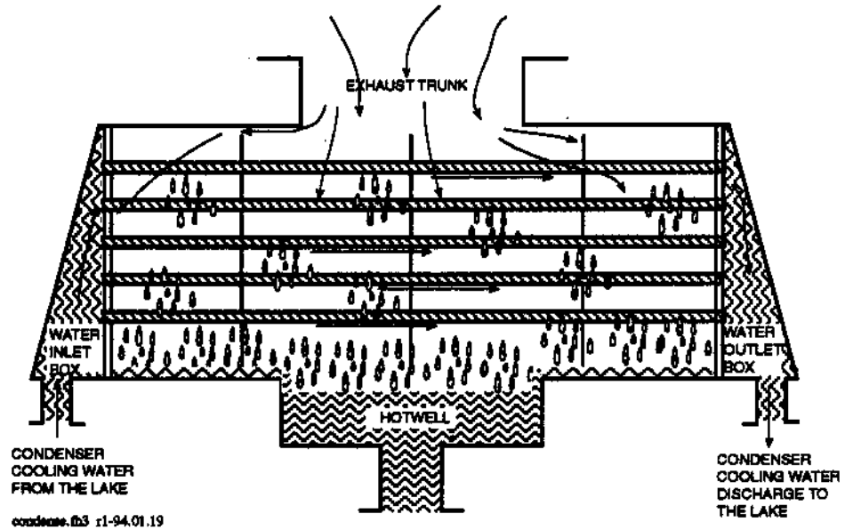
Figure 3.11 The Condenser
