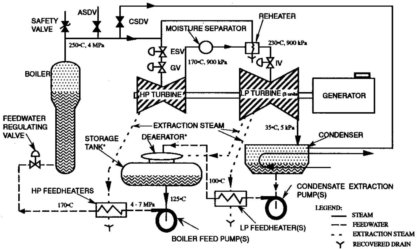
Figure 3.12 Simplified Feedheating System and Steam System
