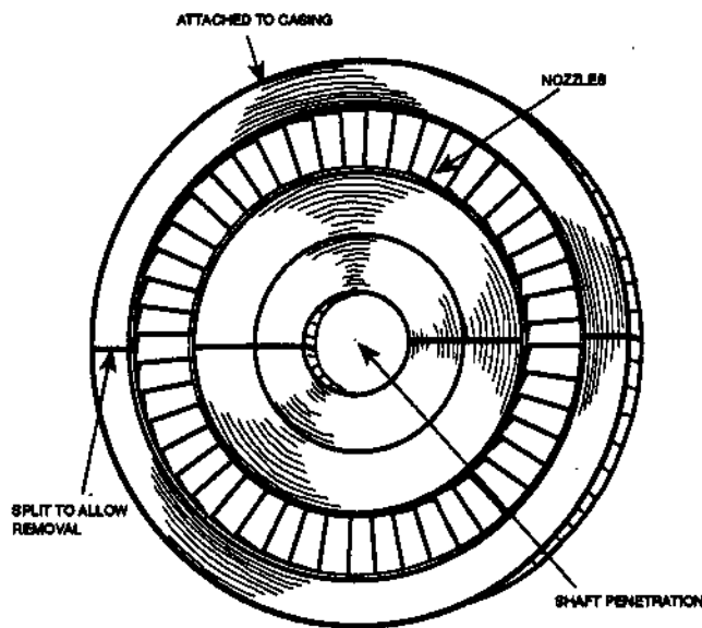
Figure 3.8 Turbine Diaphragm
