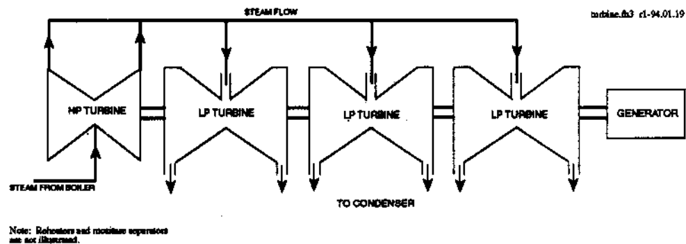
Figure 3.9 Typical Turbine Layout
