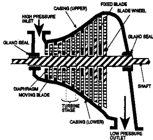
Figure 3.7 Turbine Section View
