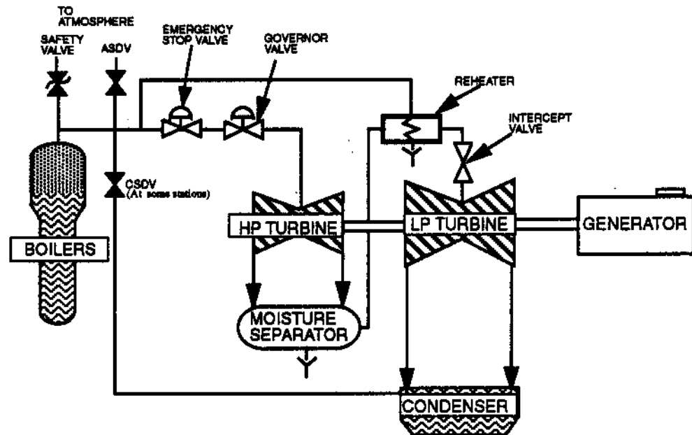
Figure 3.4 Simplified Steam System
