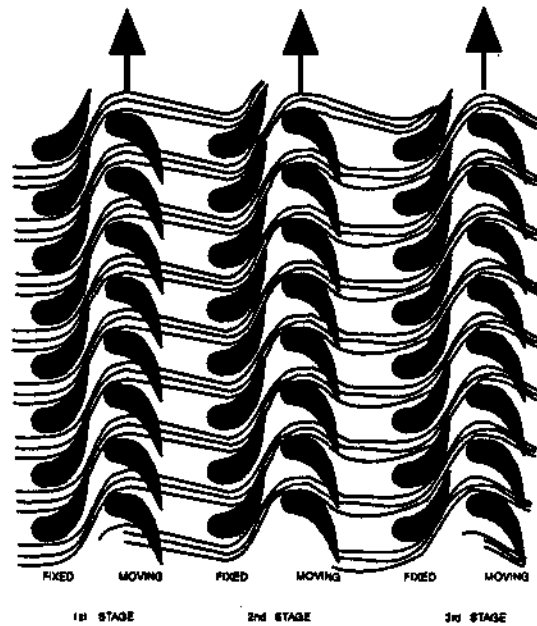
Figure 3.5 Fixed and Moving Blades Arrangement
