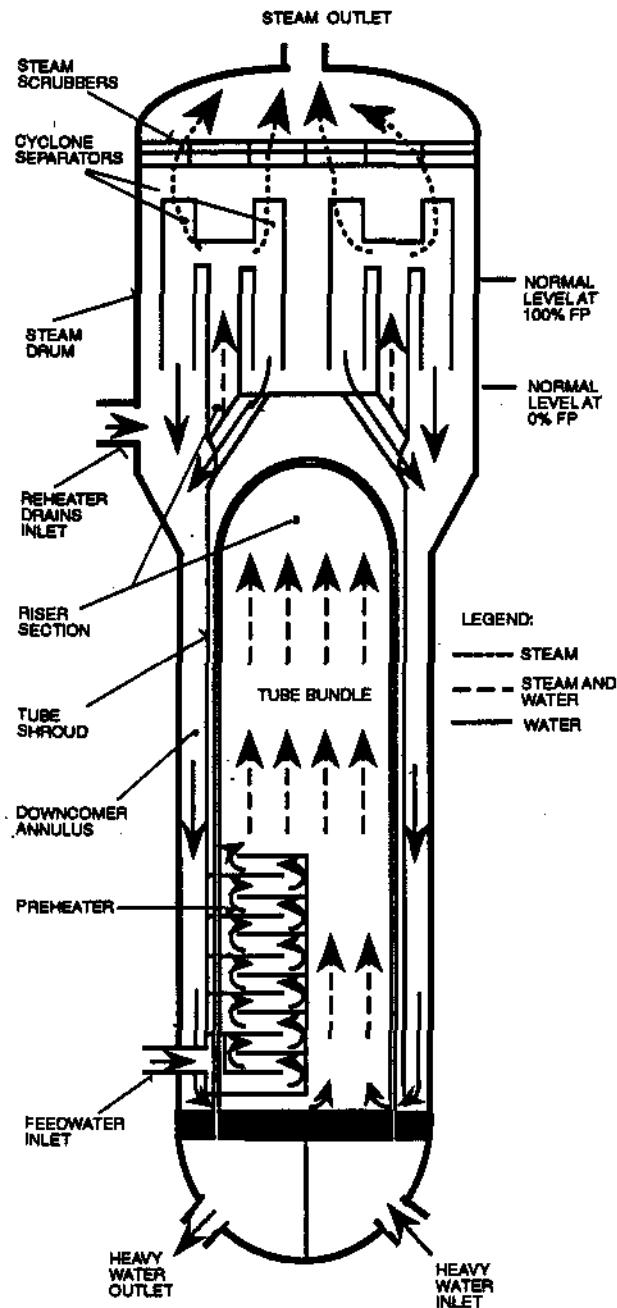
Figure 3.3 Typical Boiler
