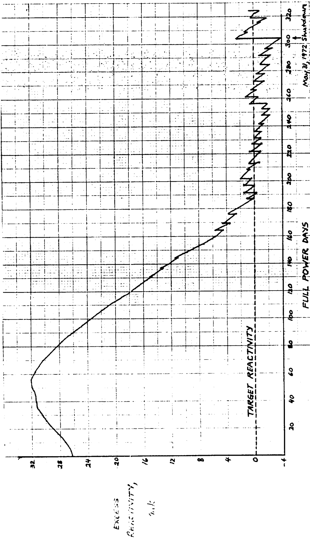
Reactivity as a Function of Burnup for Pickering Unit #1.
