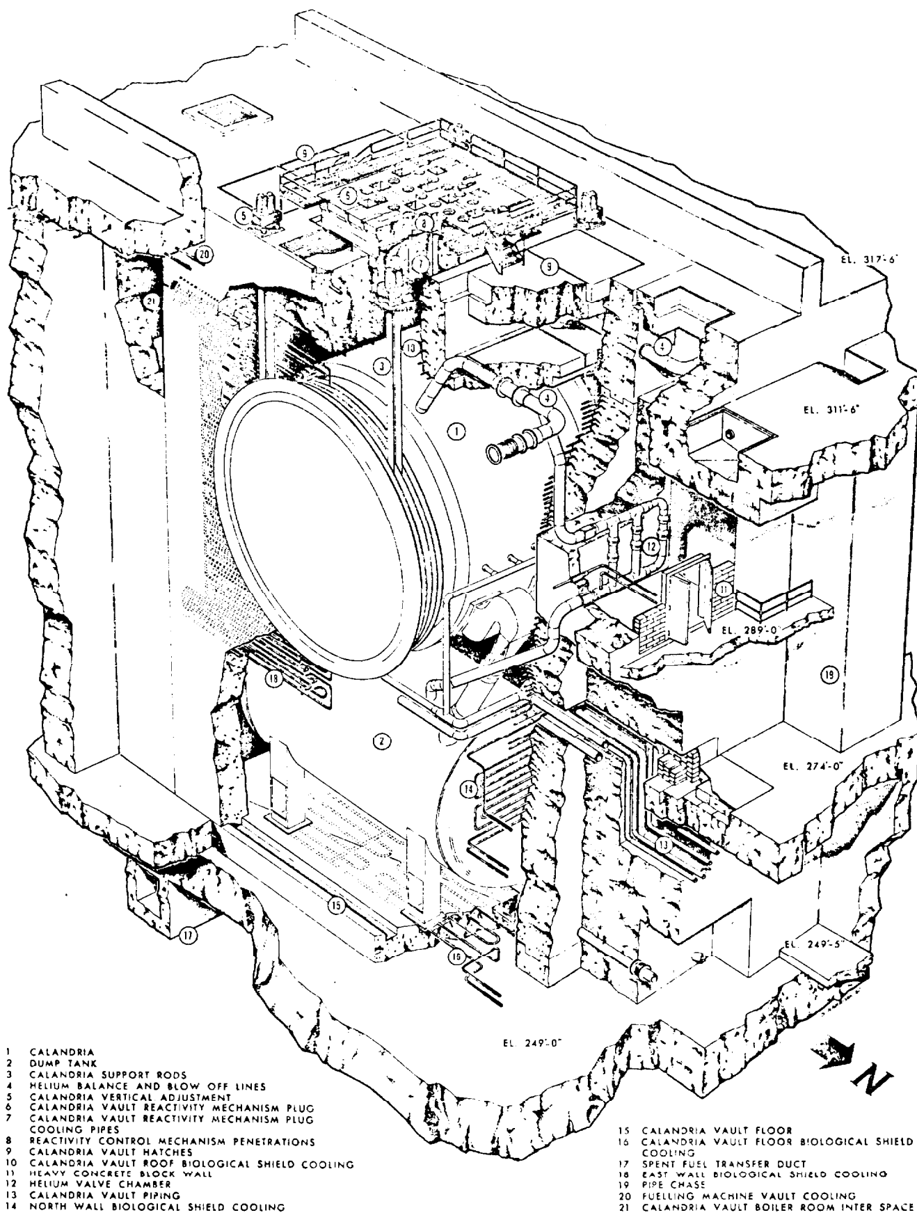
Fig. 10.6: Pickering Calandria Vault
