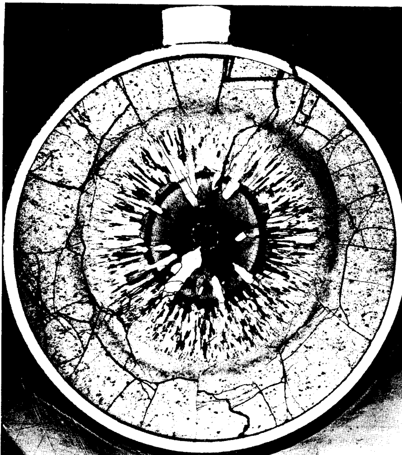
Figure 34 Cross Section of Element and Centre Melting in UO_2 Showing Defect in Fuel Element Sheath
