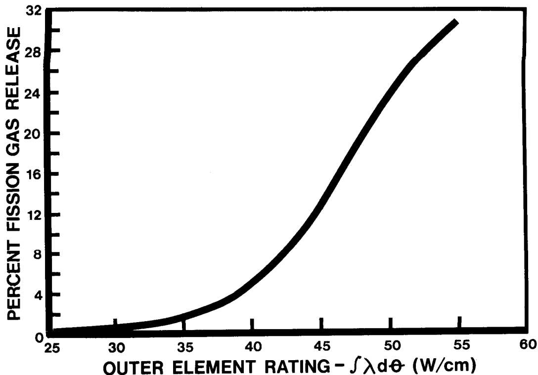
Figure 19 Percent Fission Gas Release vs UO 2 Power Rating
