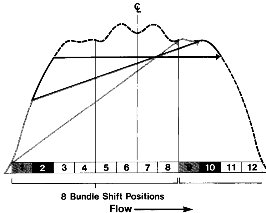
Figure 39 Pickering Axial Flux Profile
