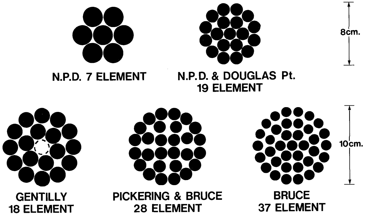
Figure 3 Fuel Bundle Cross-Sections
