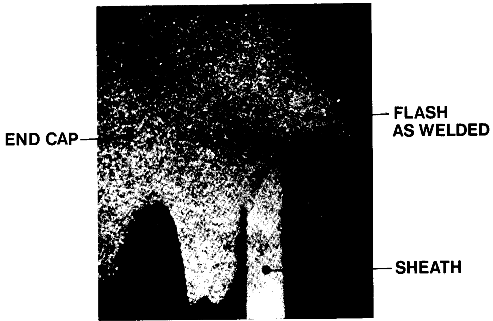
Figure 8 Cross Section Through Closure Weld
