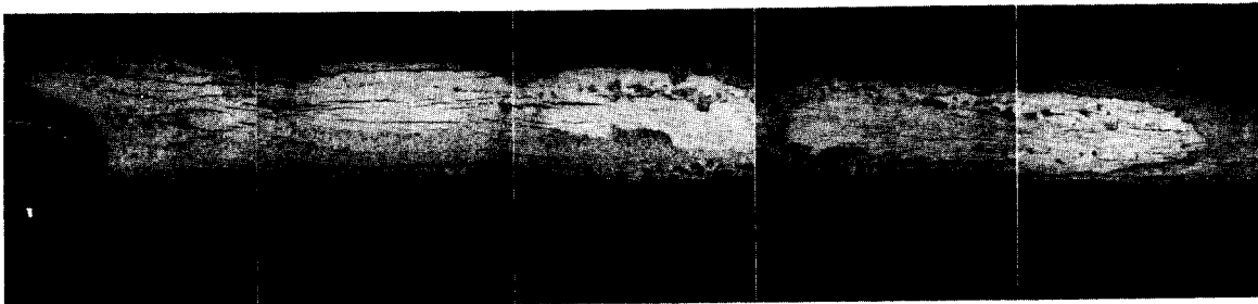
Figure 37 High Temperature Corrosion Failure of a Fuel Element
