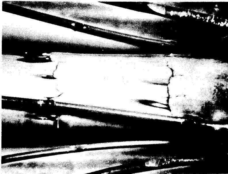
Figure 32 Douglas Point Defect Example
