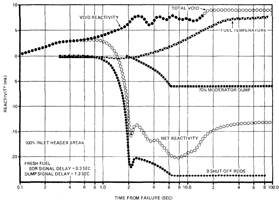
Figure 3 Reactivity Transients
