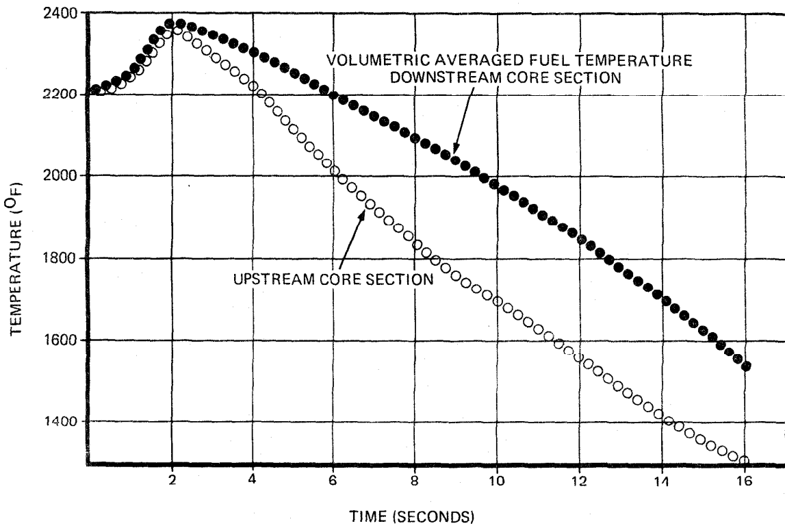
Figure 5 Fuel Temperatures
