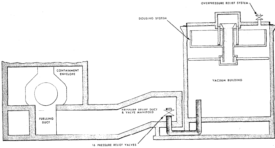
Figure 6 Vacuum Containment System
