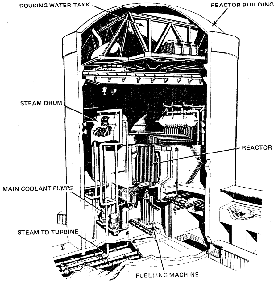
Figure 7 Gentilly Reactor Building
